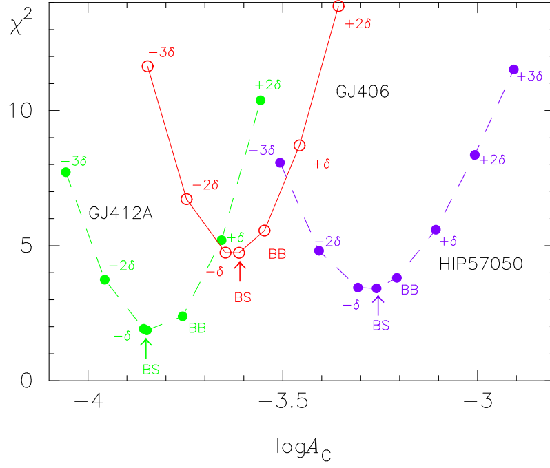
Fig. 14. \chi^2 values for the fittings of the observed and predicted spectra are plotted against \log A_C for GJ412A, GJ406, and HIP57050. In this figure, BB and BS correspond to the carbon abundances based on BB ( \log A_C(\text{BB}) ) and BS ( \log A_C(\text{BS}) ) methods, respectively, and \pm n\delta to \log A_C(\text{BB}) \pm n\delta ( n = 1, 2, \text{ and } 3 ). Note that the results by the BS analysis are almost at the minima but those by the BB analysis are still not.
