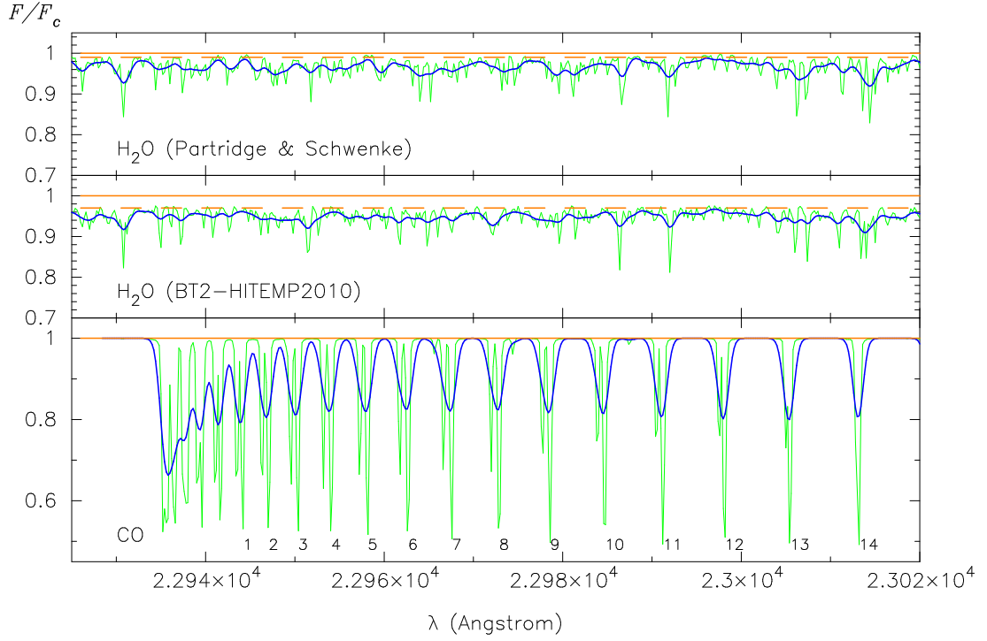
Fig. 4. Theoretical spectra for the model Cc3500c475. The spectra are first calculated with a sampling interval of 0.02 \text{ \AA} (thin lines) and then they are convolved with the slit function of \text{FWHM} = 16 \text{ km sec}^{-1} (thick lines). The true- and pseudo-continuous levels are shown by the solid and dashed lines, respectively. a) \text{H}_2\text{O} spectrum based on the line-list by Partridge & Schwenke (1997). b) \text{H}_2\text{O} spectrum based on the line-list BT2-HITEMP2010 (Barber et al. 2006; Rothman et al. 2010). c) CO spectrum near the (2,0) band head. The reference numbers of table 7 are given to respective CO blends.
