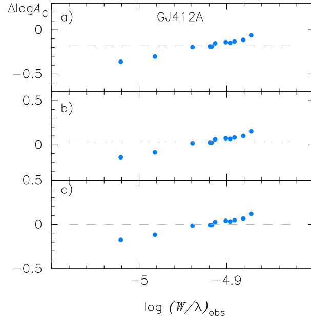
Fig. 5. The resulting logarithmic abundance corrections by the BB analysis for the CO lines in GJ412A plotted against the observed values of \log W/\lambda . The dashed line shows the mean correction. a) First iteration. b) Second iteration. c) Confirmation of the convergence.
