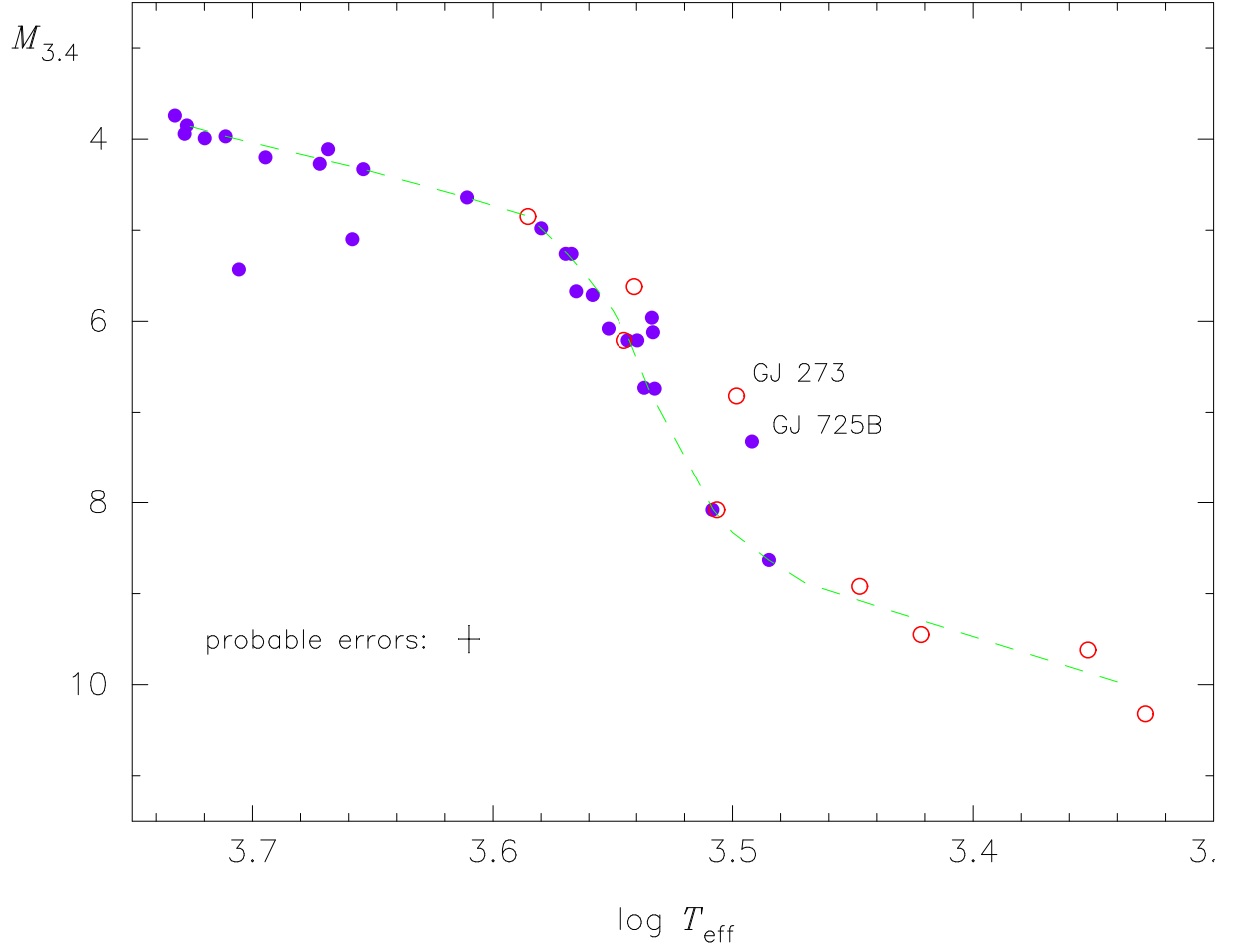
Fig. 1. The absolute magnitude at 3.4\mu\text{m} , M_{3.4} , plotted against \log T_{\text{eff}} , where T_{\text{eff}} values are based on the interferometry (filled circles) and infrared flux method (open circles). The dashed line is a mean curve. The probable errors of T_{\text{eff}} , reproduced from Table 6 of Boyajian et al. (2012) to our table 3, are less than 1% for 21 objects out of 27 objects and only one object shows larger than 2% error in the remaining 6 objects. The probable errors of M_{3.4} are less than 0.15 mag for 22 objects out of 27 objects (see table 3). The error bars representing 1% probable error in T_{\text{eff}} and probable error of 0.15 mag in M_{3.4} are shown at the lower left corner.
