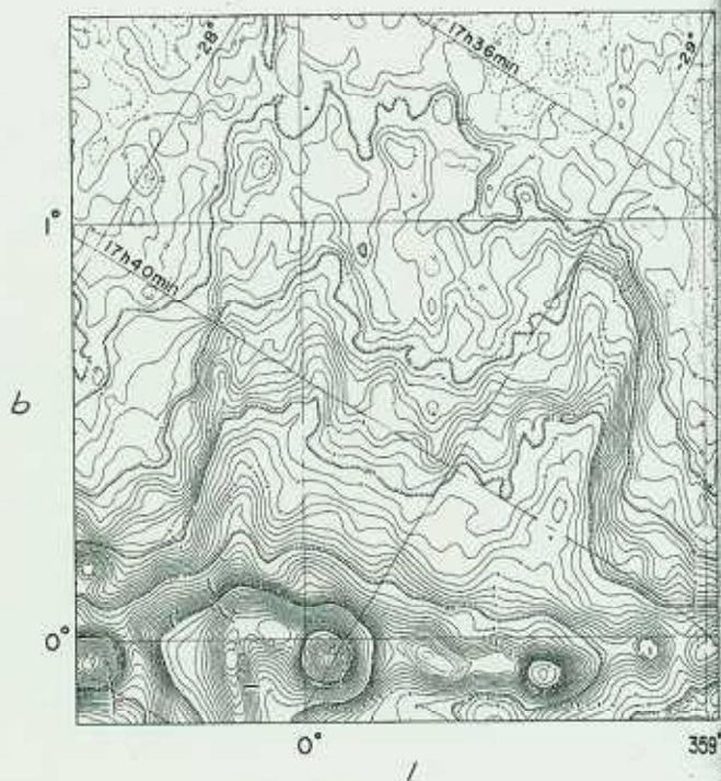
Fig. 1 A 10.5-GHz radio continuum map of the galactic centre region showing the whole structure of the GCL. The map has been convoluted to a 3.6 arc min HPBW gaussian beam. The numbers on contours are in unit of 5.77 mJy per beam of 2.6 arc min HPBW ( = 9.1 \times 10^{-23} \text{ W m}^{-2} \text{ Hz}^{-1} \text{ sr}^{-1} = 2.7 \text{ mK } T_b ).
