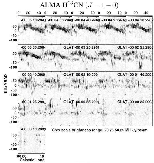
Fig. 19. [Top] Channel LVDs in HCN ( J = 4 - 3 ) by ASTE 10-m telescope. [Middle] ACES latitude-channel maps of LVDs in CS ( J = 2 - 1 ) (top) and [bottom] H^{13}CN ( J = 1 - 0 ) (bottom) of the central \pm 0^\circ.12 about Sgr A*. Alt text: Latitudinal channel LVDs in HCN ( J = 4 - 3 ) from ASTE-10 m, channel LVDs in CS ( J = 2 - 1 ) and H^{13}CN ( J = 1 - 0 ) by ACES.
