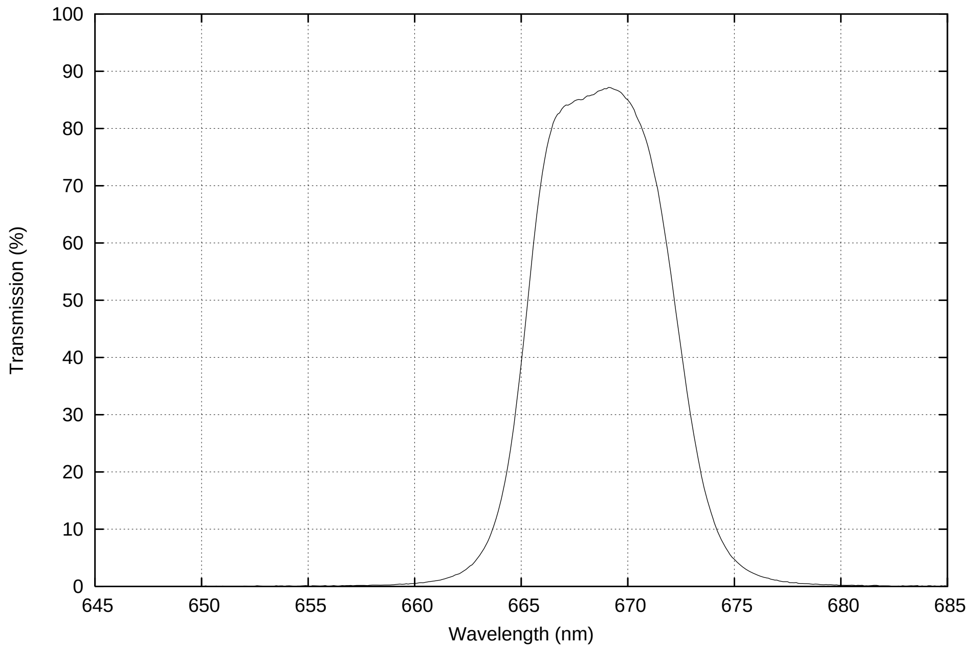
6680 filter Transmission data 2009/03/18
