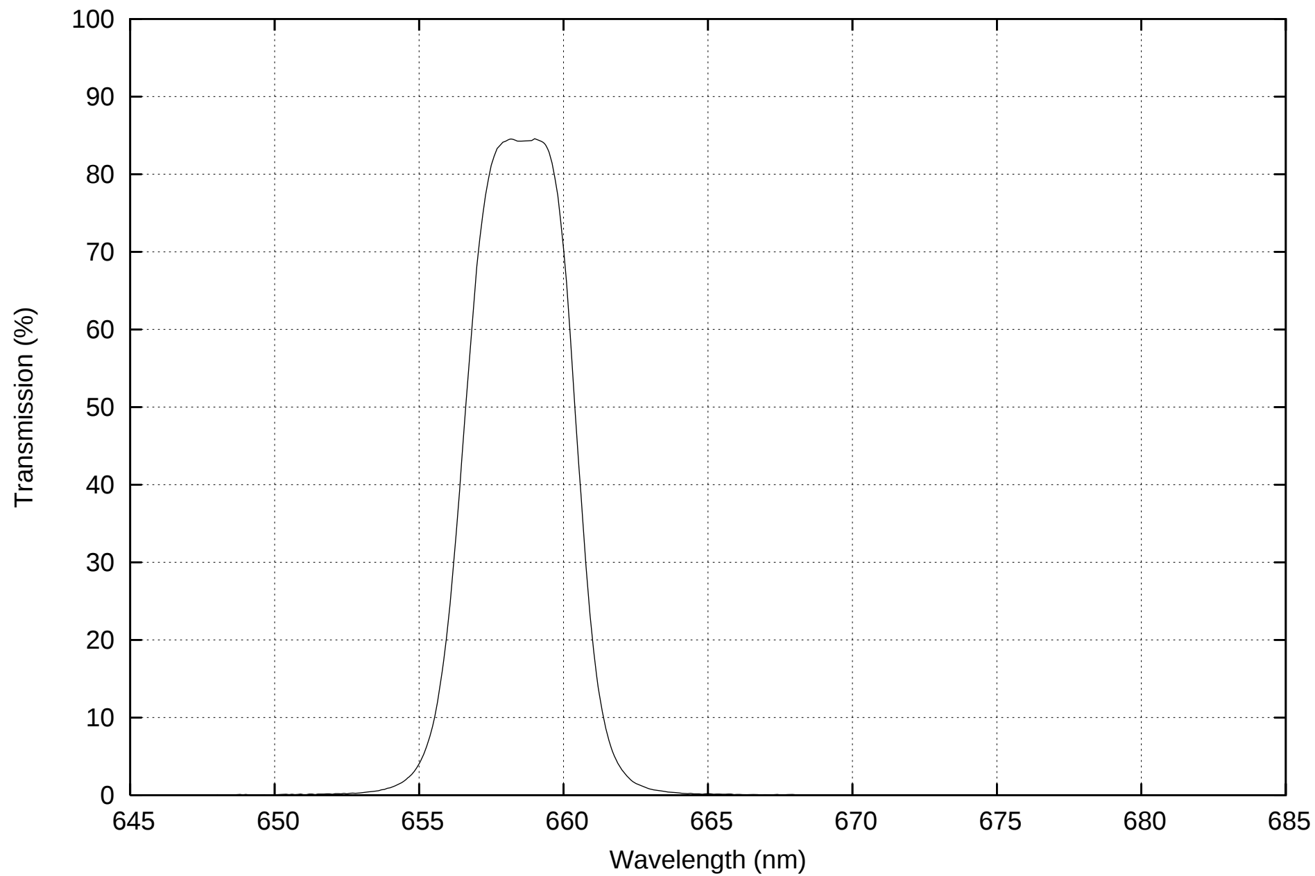
6577 filter Transmission data 2009/03/18
