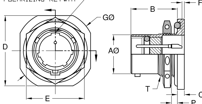
DT02H - FLANGE MOUNT CONNECTORS (MIL-STD-3112H TYPE)
