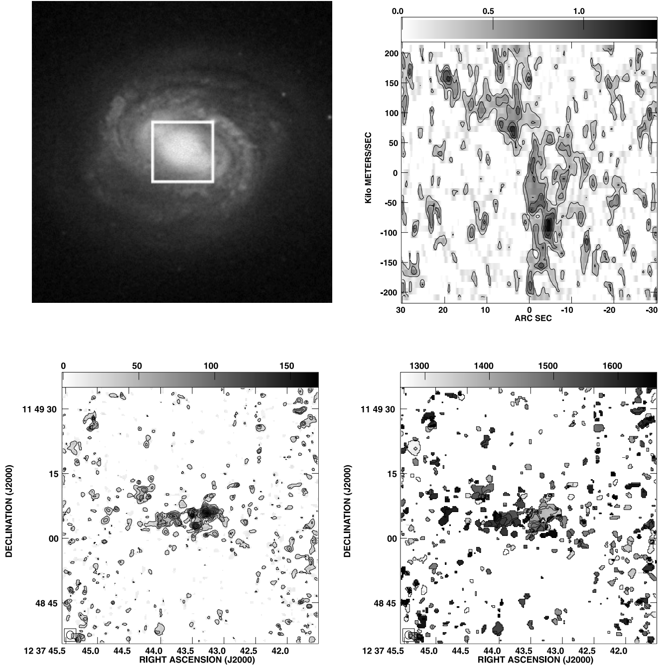
Fig. 1. (Continued.) (l) NGC 4579: (tl) DSS b -band 5' \times 5' ; i = 37^\circ ; PA = 60^\circ . (bl) Ico: 1' \times 1' ; cl = 20 \times (1, 2, 3, \dots, 7) Kkm s ^{-1} . (tr) PVD: 1' \times 5' , PA = 90^\circ ; cl = 0.25 \times (1, 2, \dots, 6) K. (br) V-field: 1' \times 1' ; cl = 1320 to 1600, every 20 km s ^{-1} .
