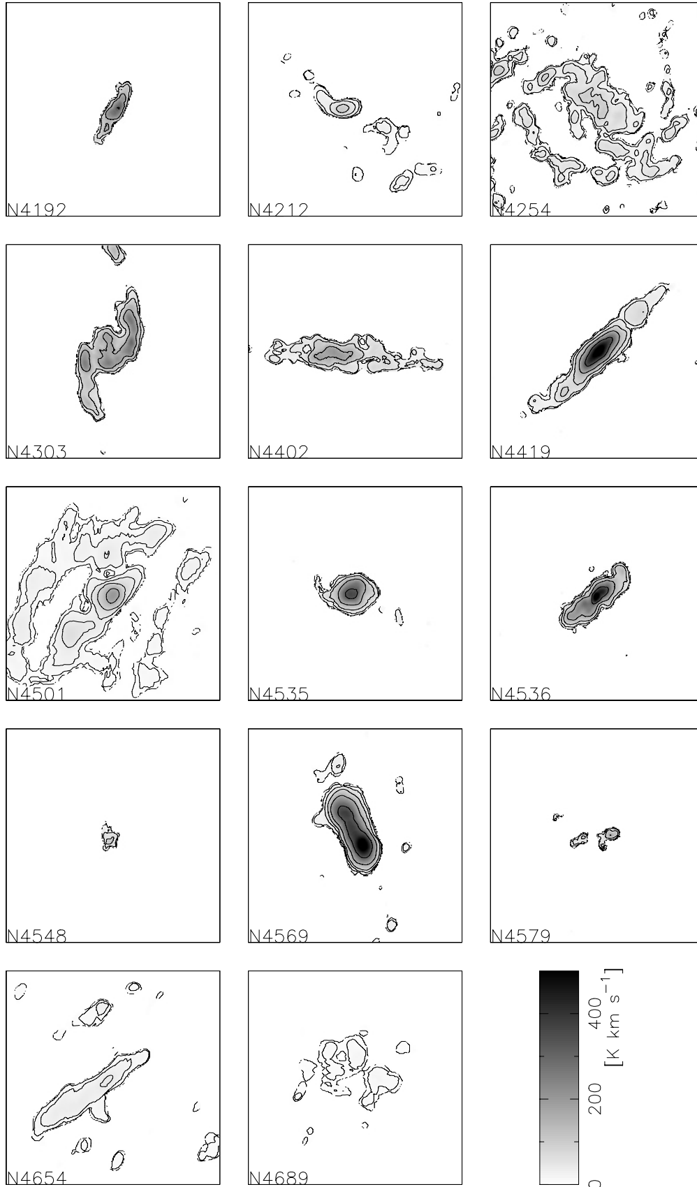
Fig. 2. Integrated ^{12}\text{CO} ( J=1-0 )-intensity maps of the observed galaxies in the same angular scale. The image sizes are 1'.0 \times 1'.0 , or 4.68 \text{ kpc} \times 4.68 \text{ kpc} for an assumed distance of 16.1 Mpc. The contours are drawn at 5, 10, 20, 40, 80, and 160 \text{ K km s}^{-1} .
