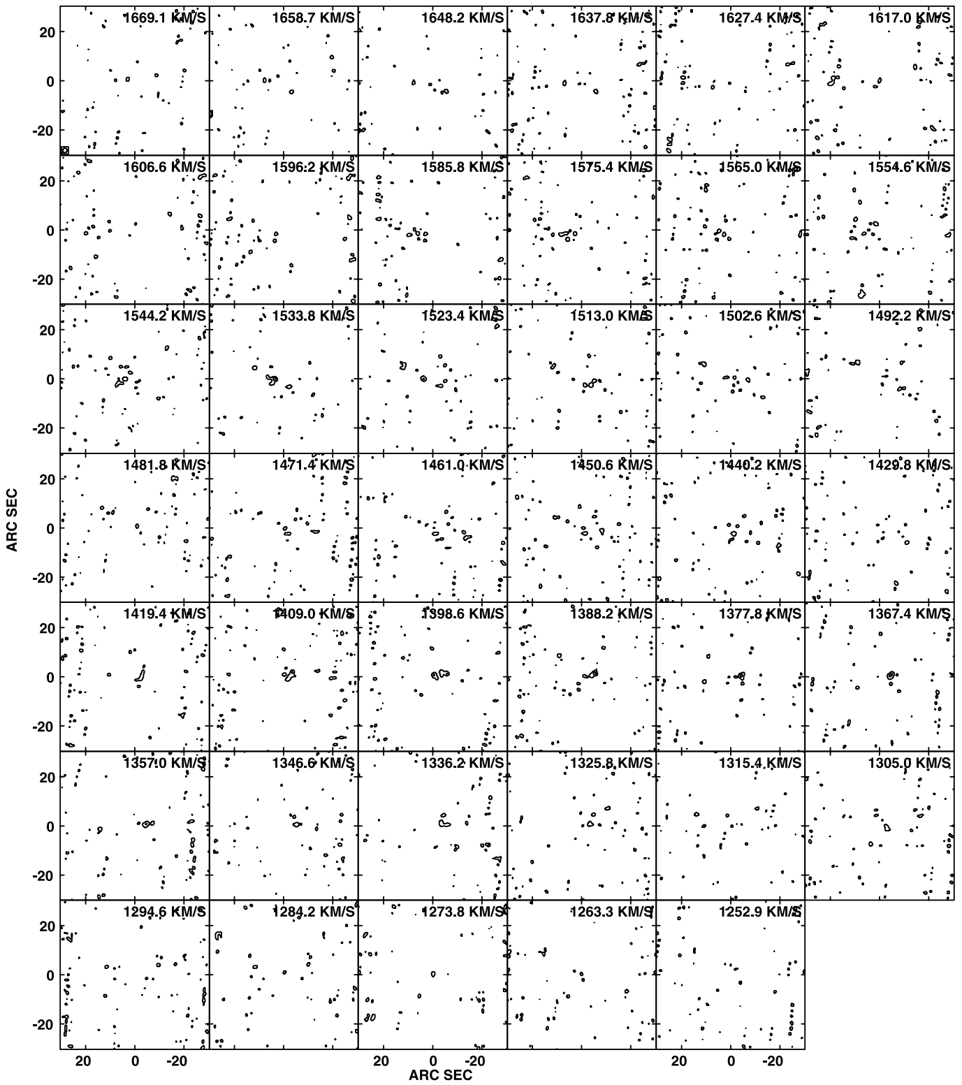
Fig. A1. (Continued.) NGC 4579: Lowest c_1 = 1.0K .
