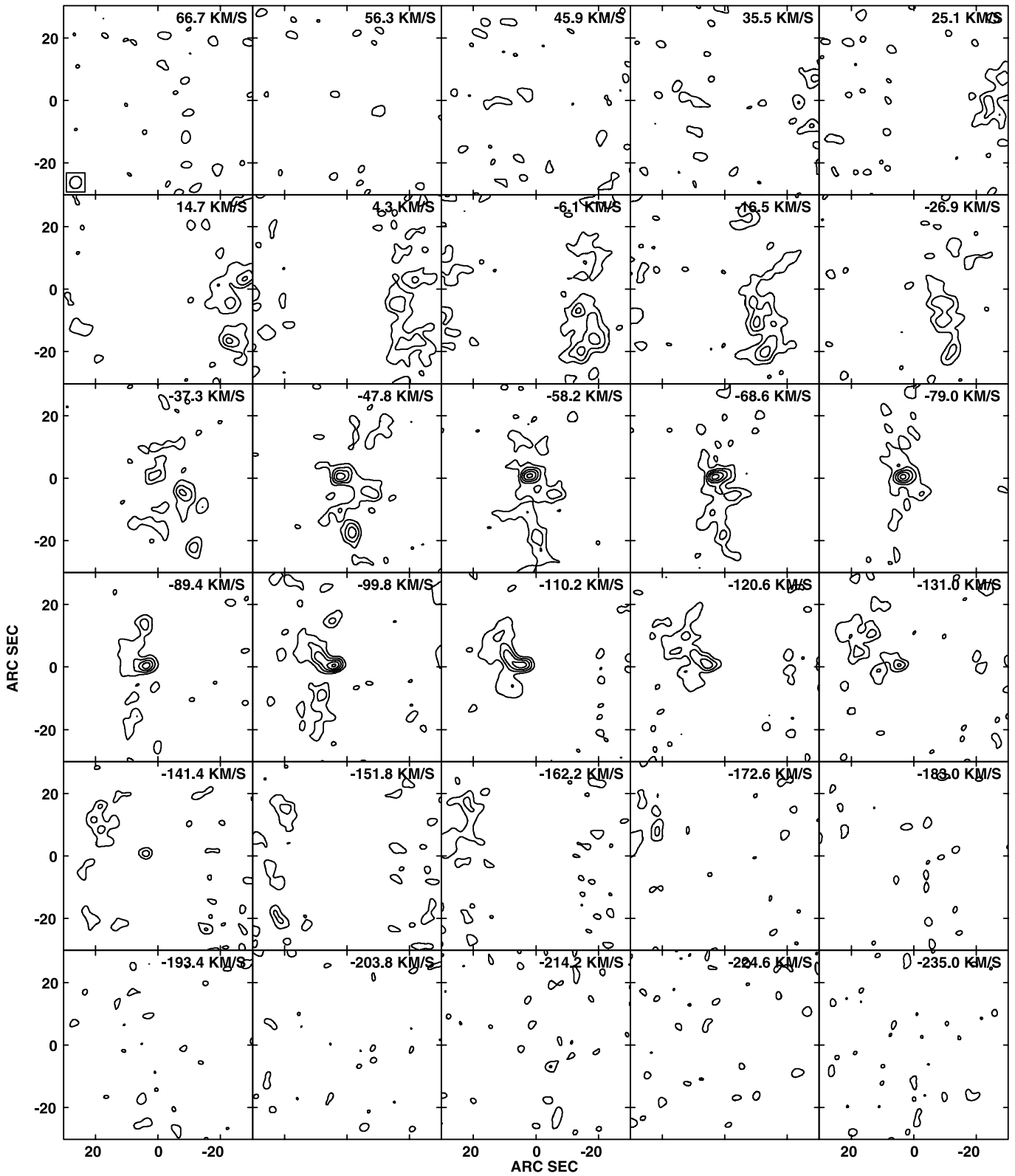
Fig. A1. (Continued.) NGC 4212: Lowest \text{cl} = 0.25 \text{ K} .
