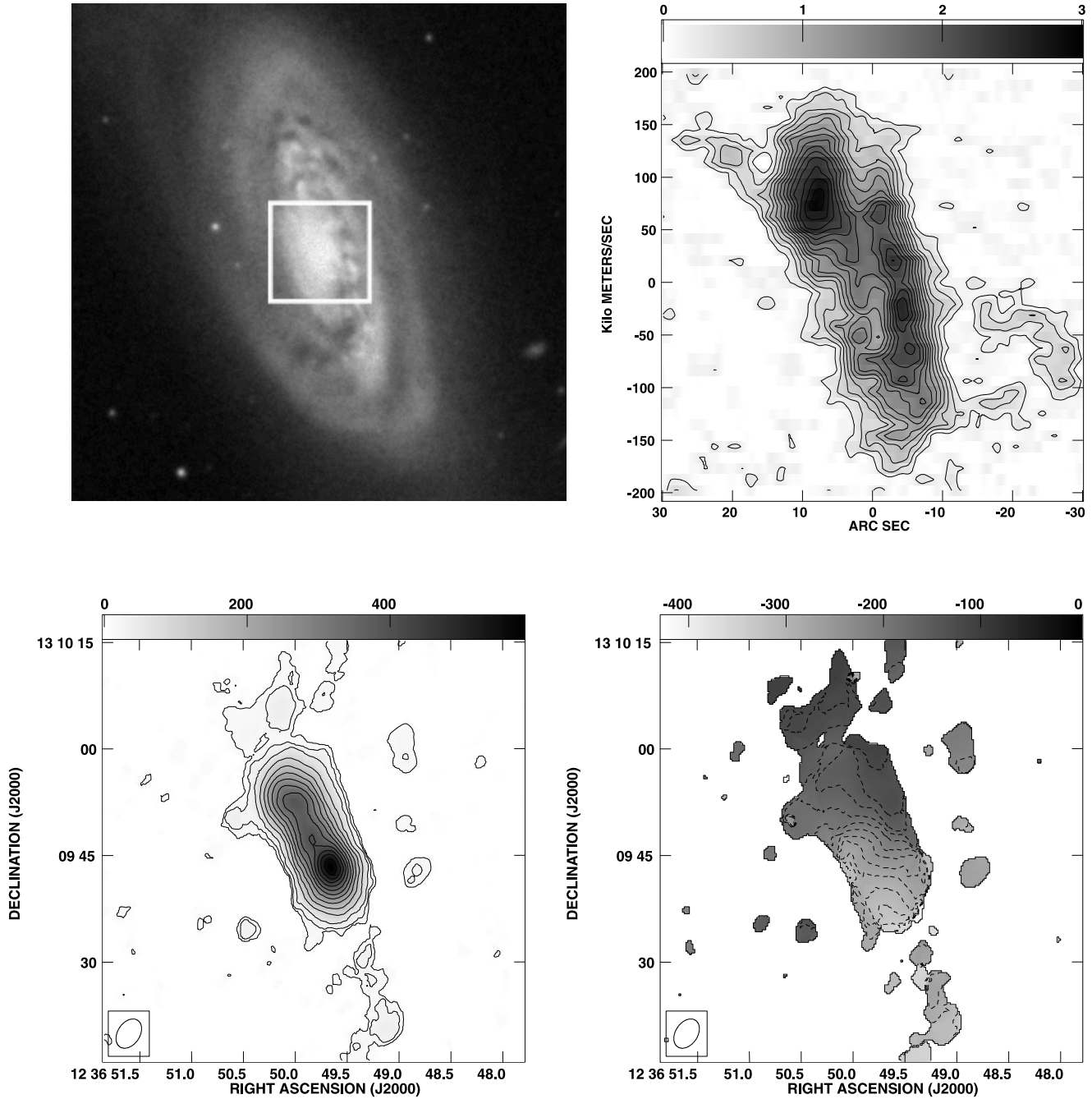
Fig. 1. (Continued.) (k) NGC 4569: (tl) DSS b -band 5' \times 5' ; i = 63^\circ ; PA = 23^\circ . (bl) Ico: 1' \times 1' ; cl = 50 \times (0.25, 0.5, 1, 2, \dots, 12) K km s ^{-1} . (tr) PVD: 1' \times 5' , PA = 160^\circ ; cl = 0.2 \times (1, 2, \dots, 15) K. (br) V-field: 1' \times 1' ; cl = -380 to 0 , every 20 km s ^{-1} .
