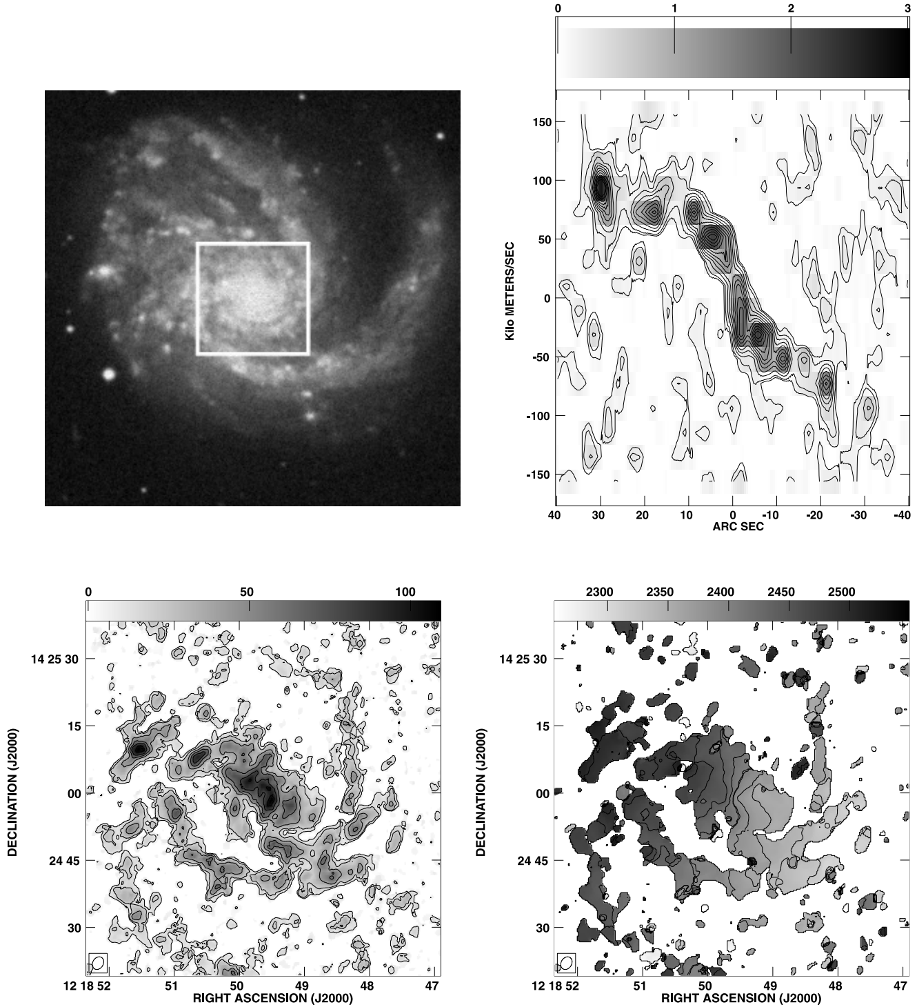
Fig. 1. (Continued.) (c) NGC 4254: (tl) DSS b -band 5' \times 5' , i = 42^\circ , PA = 45^\circ . (bl) Ico: 80'' \times 80'' ; cl = 10 \times (1, 2, \dots, 12) K km s ^{-1} . (tr) PVD: 1' \times 3'' , PA = 45^\circ ; cl = 0.132 \times (1, 2, \dots, 12) K. (br) V-field: 1' \times 1' ; cl = 2300 to 2530, every 20 km s ^{-1} .
