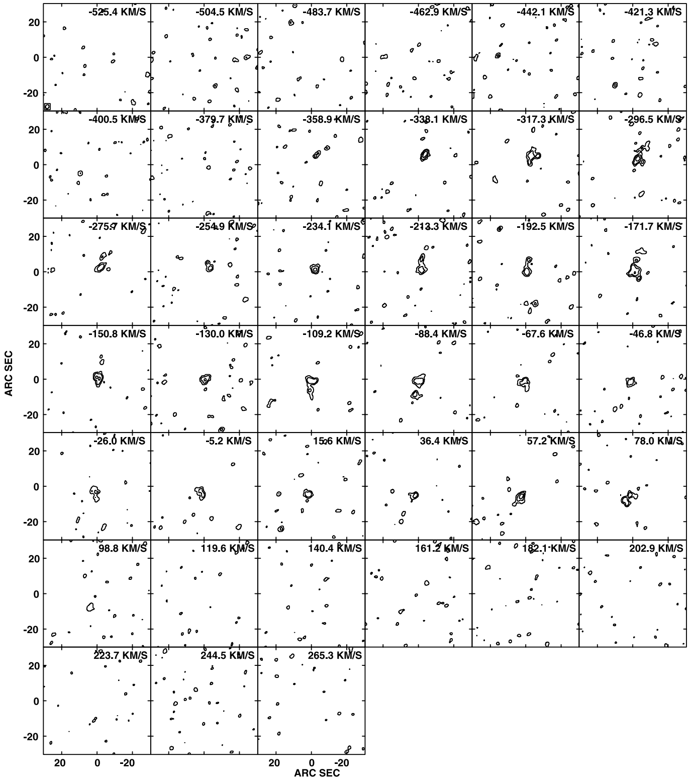
Fig. A1. Channel maps of the ^{12}\text{CO} ( J = 1-0 ) line emission of the Virgo galaxies. Intensity scale is in Kelvin of brightness temperature. Contours are drawn at 2^n times the lowest-contour value ( n = 1, 2, 3, \dots ). The lowest contour level (cl) is indicated for individual galaxies. NGC 4192: Lowest cl (contour level) = 0.5 K.
