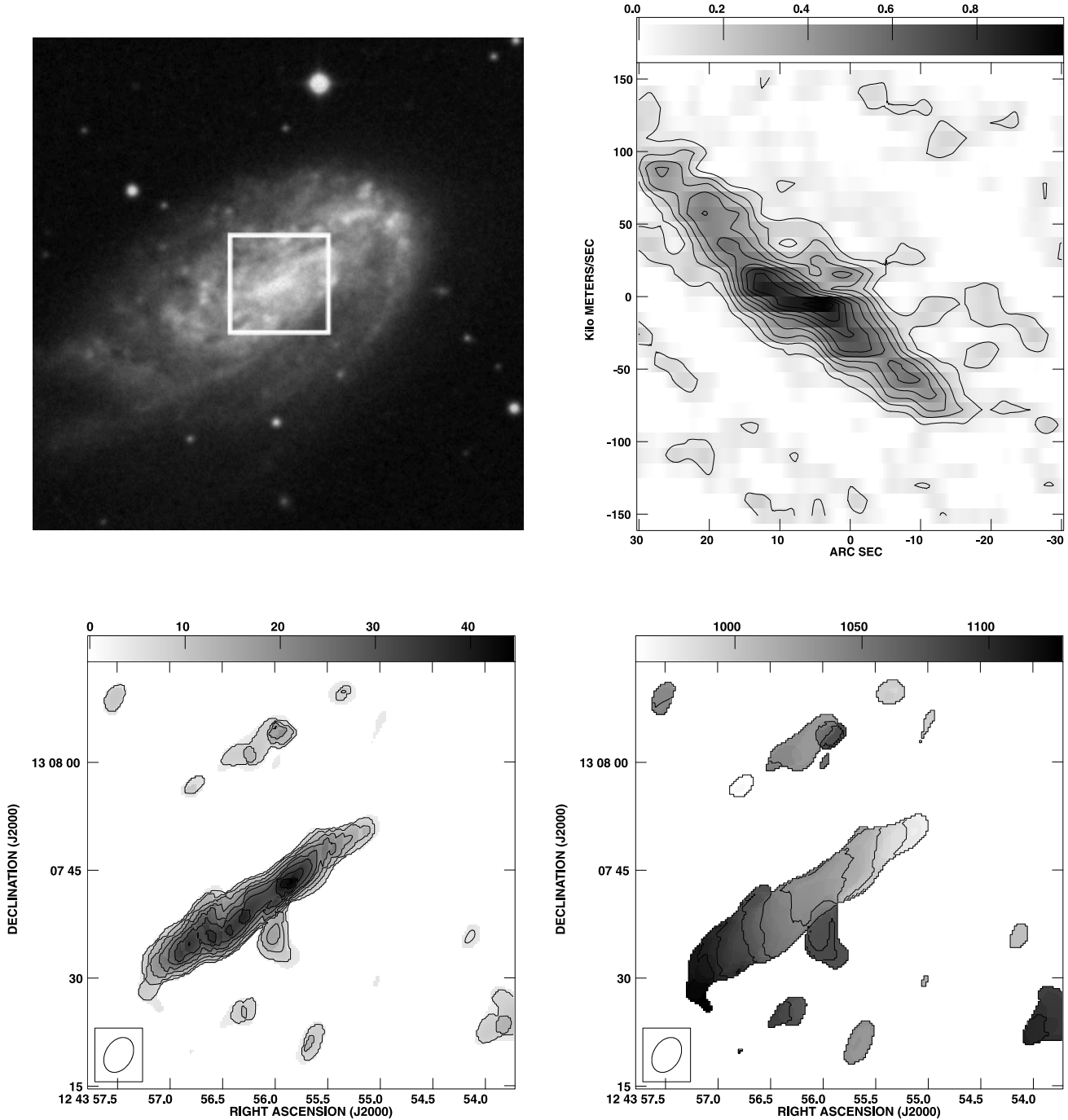
Fig. 1. (Continued.) (m) NGC 4654: (tl) DSS b -band 5' \times 5' ; i = 51^\circ ; PA = 128^\circ . (bl) Ico: 1' \times 1' ; cl = 5 \times (1, 2, \dots, 10) Kkms ^{-1} . (tr) PVD: 1' \times 3' , PA = 128^\circ ; cl = 0.1 \times (1, 2, \dots, 10) K. (br) V-field: 1' \times 1' ; cl = 960 to 1120, every 20kms ^{-1} .
