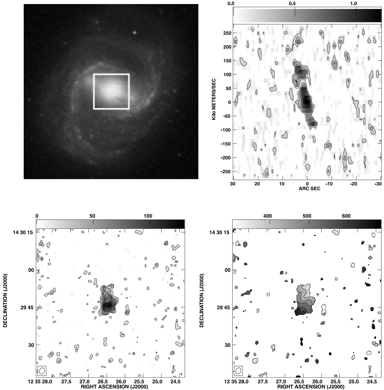
Fig. 1. (Continued.) (j) NGC 4548: (tl) DSS b -band 5' \times 5' ; i = 37^\circ ; PA = 150^\circ . (bl) Ico: 1' \times 1' ; cl = 10 \times (1, 2, 3, \dots, 12) \text{ K km s}^{-1} . (tr) PVD: 1' \times 5'' , PA = 150^\circ ; cl = 0.15 \times (1, 2, \dots, 10) \text{ K} . (br) V-field: 1' \times 1' ; cl = 300 \text{ to } 700 , every 50 \text{ km s}^{-1} .
