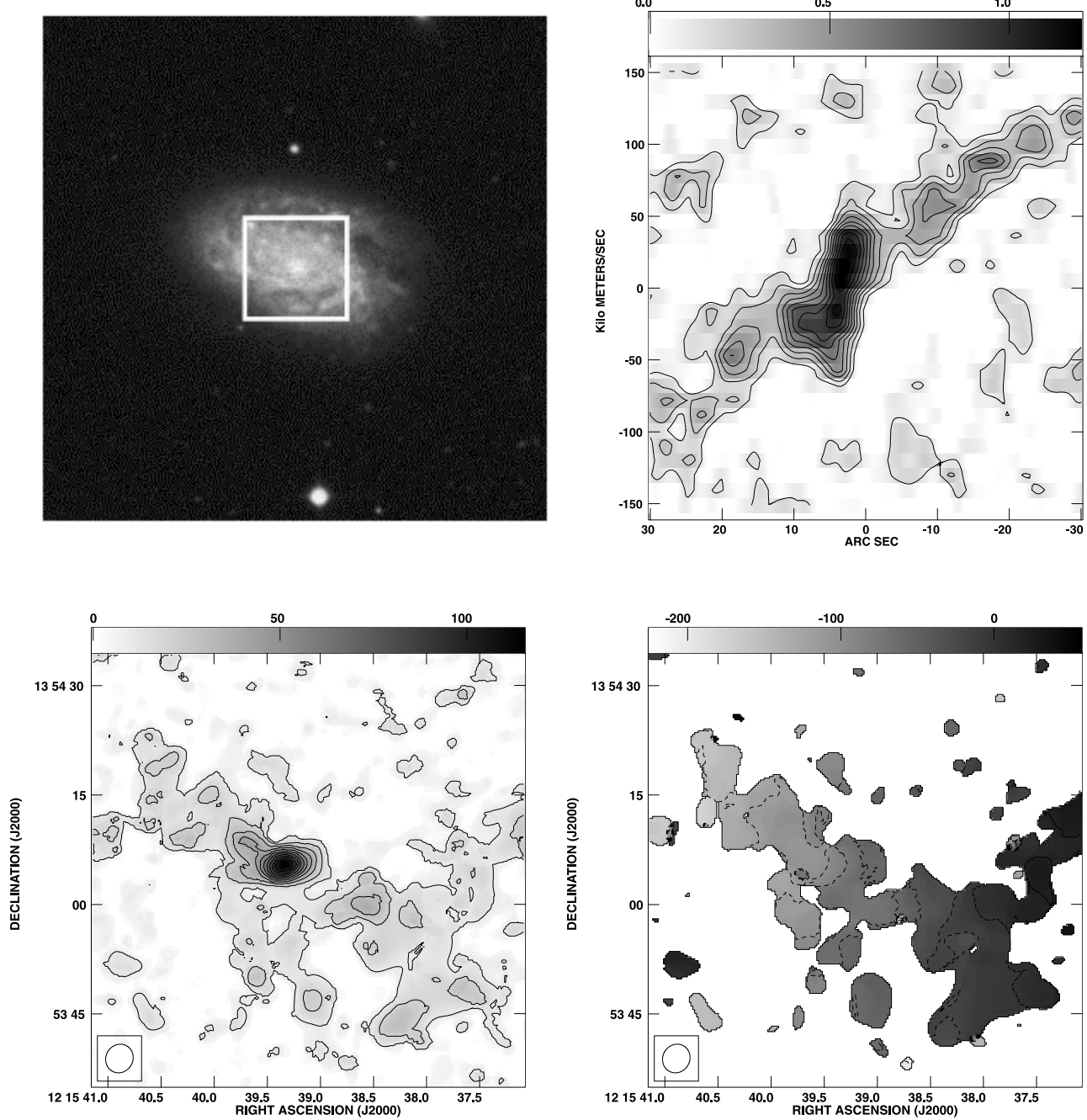
Fig. 1. (Continued.) (b) NGC 4212: (tl) DSS b -band 5' \times 5' ; i = 47^\circ ; PA = 75^\circ . (bl) Ico: 1' \times 1' ; cl = 50 \times (0.5, 1, 2, 3, \dots, 10) \text{K km s}^{-1} . (tr) PVD: 1' \times 3'' , PA = 75^\circ ; cl = 0.5 \times (0.25, 1, 2, \dots, 10) \text{K} . (br) V-field: 1' \times 1' ; cl = -200 to 40 , every 20 \text{ km s}^{-1} .
