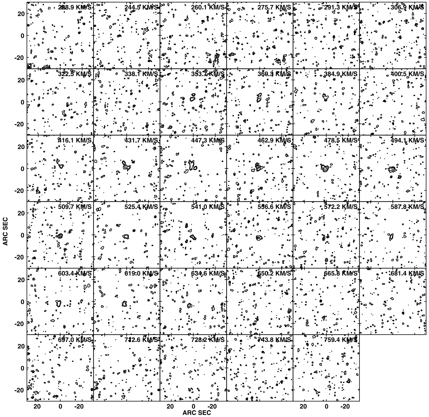
Fig. A1. (Continued.) NGC 4548: Lowest \sigma_l = 0.25 K.
