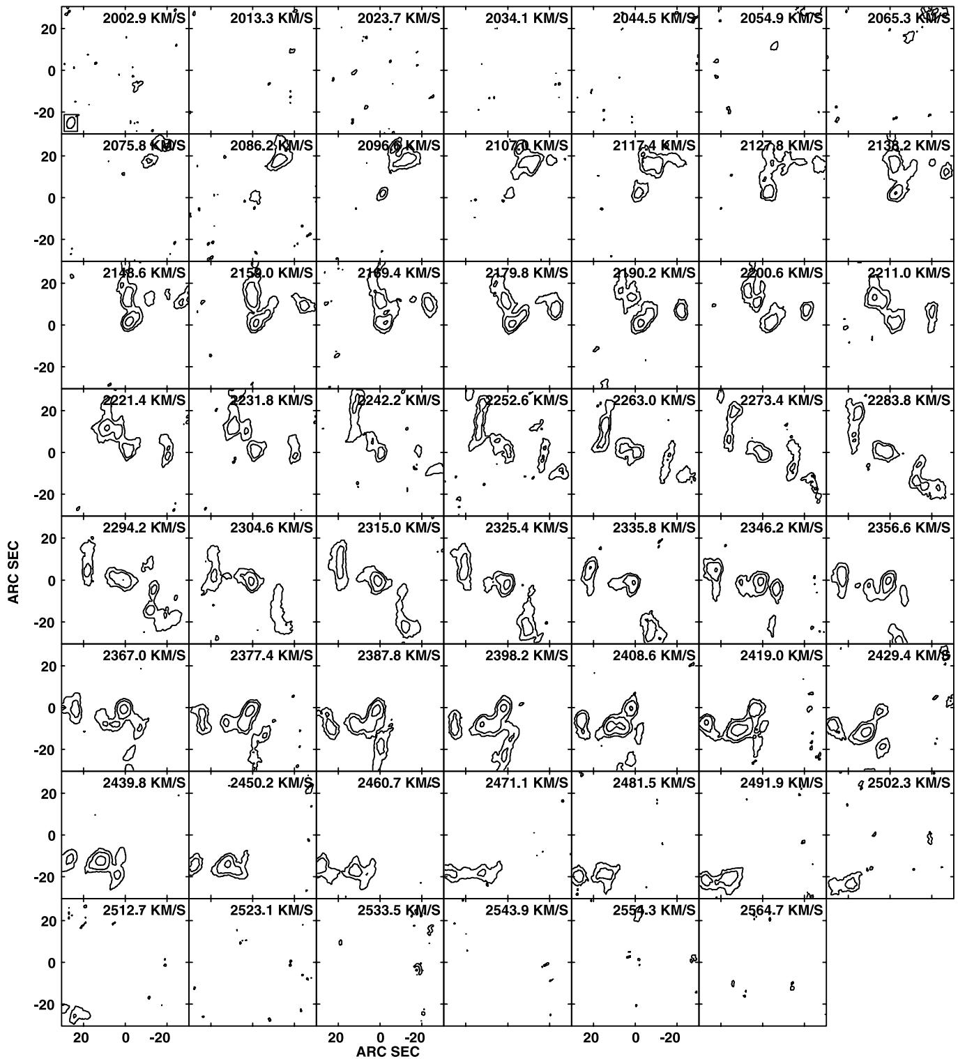
Fig. A1. (Continued.) NGC 4501: Lowest \text{cl} = 0.20\text{K} .
