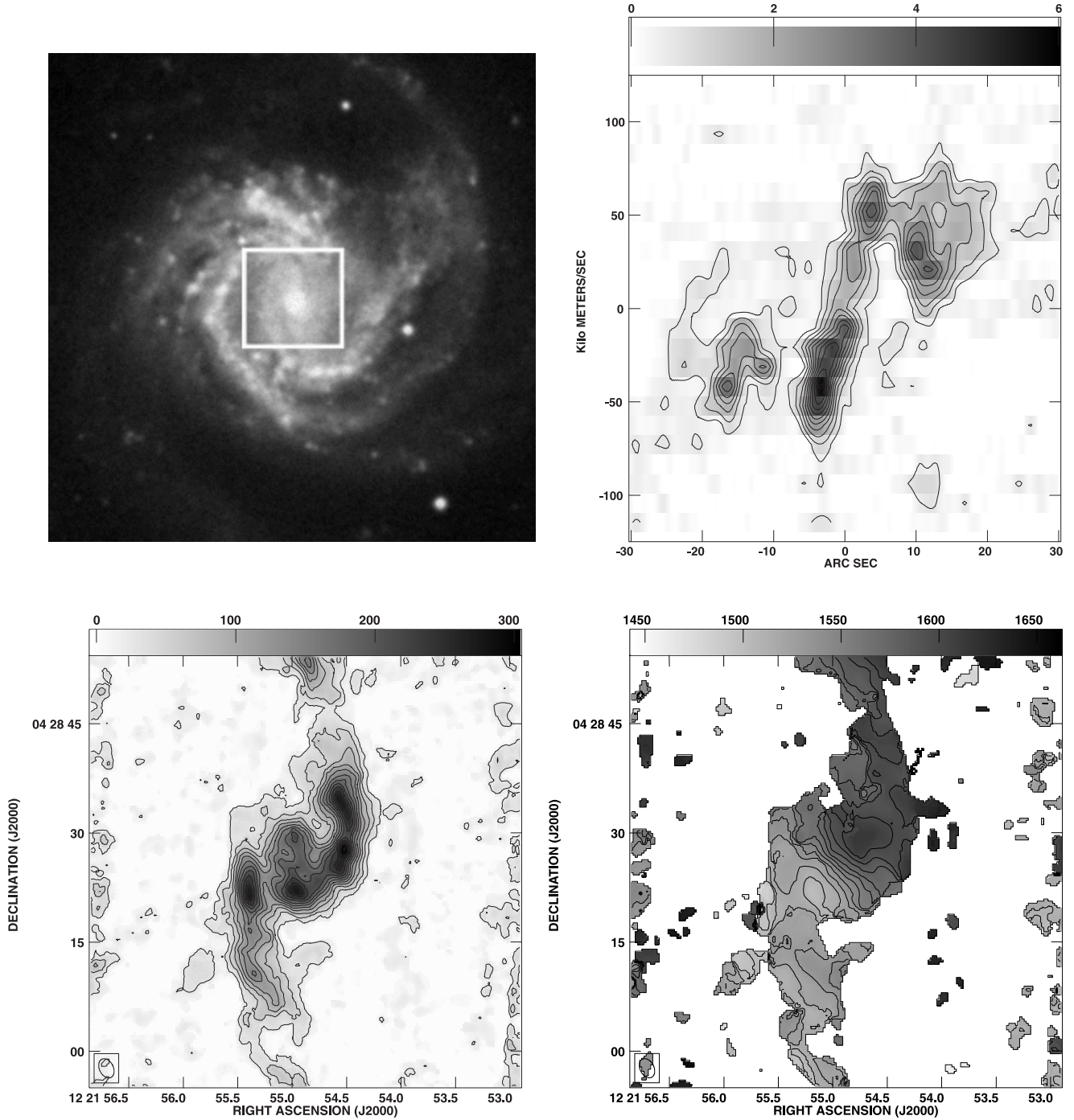
Fig. 1. (Continued.) (d) NGC 4303: (tl) DSS b -band 5' \times 5' , i = 25^\circ , PA = 0^\circ . (bl) Ico: 1' \times 1' ; Beam 2''.80 \times 1''.90 ; cl = 25 \times (1, 2, \dots, 12) \text{ K km s}^{-1} . (tr) PVD: 1' \times 3' , PA = 340^\circ ; cl = 0.5 \times (1, 2, \dots, 12) \text{ K} . (br) V-field: 1' \times 1' ; cl = 1500 to 1600 , every 10 \text{ km s}^{-1} .
