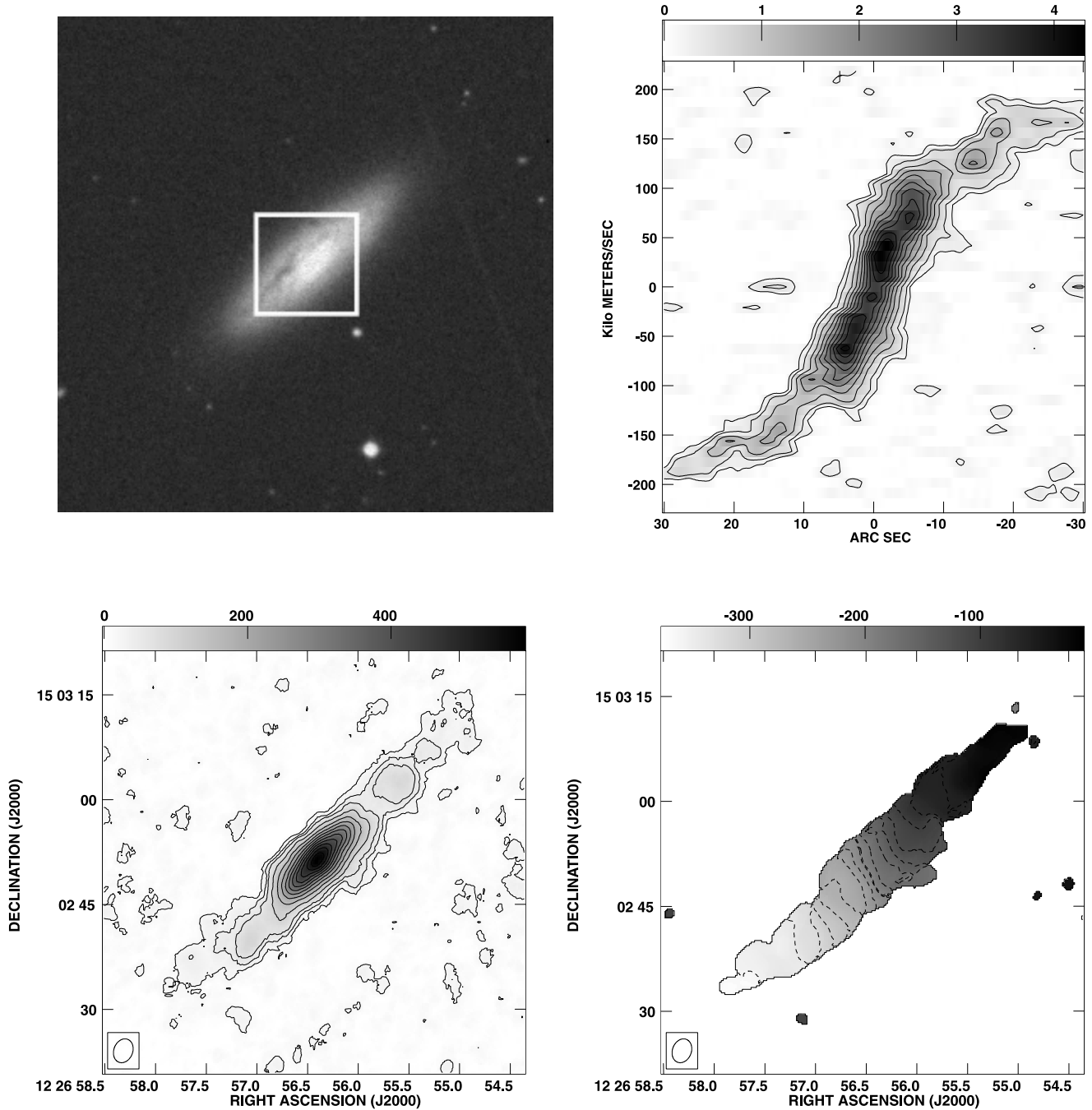
Fig. 1. (Continued.) (tl) DSS b -band 5' \times 5' ; i = 67^\circ ; PA = 133^\circ . (bl) Ico: 1' \times 1' ; cl = 50 \times (0.4, 0.8, 1.2, 2, 3, \dots, 12) K km s ^{-1} . (tr) PVD: 1' \times 5'' , PA = 133^\circ ; cl = 0.5 \times (0.5, 1, 2, \dots, 10) K. (br) V-field: 1' \times 1' ; cl = -400 to 0 , every 20 km s ^{-1} .
