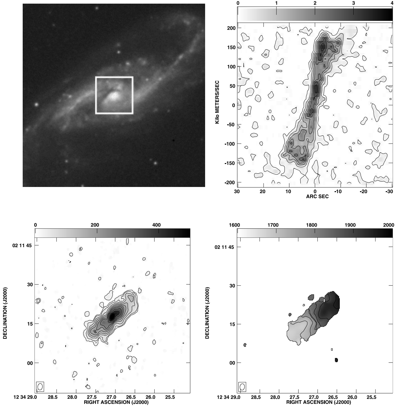
Fig. 1. (Continued.) (i) NGC 4536: (tl) DSS b -band 5' \times 5' ; i = 67^\circ ; PA = 116^\circ . (bl) Ico: 1' \times 1' ; cl = 20 \times (1, 2, 4, 6, \dots, 10, 15, 20, 25, 30) Kkms ^{-1} . (tr) PVD: 1' \times 5'' , PA = 116^\circ ; cl = 0.5 \times (0.25, 1, 2, \dots, 10) K. (br) V-field: 1' \times 1' ; cl = 1600 to 2000, every 50kms ^{-1} .
