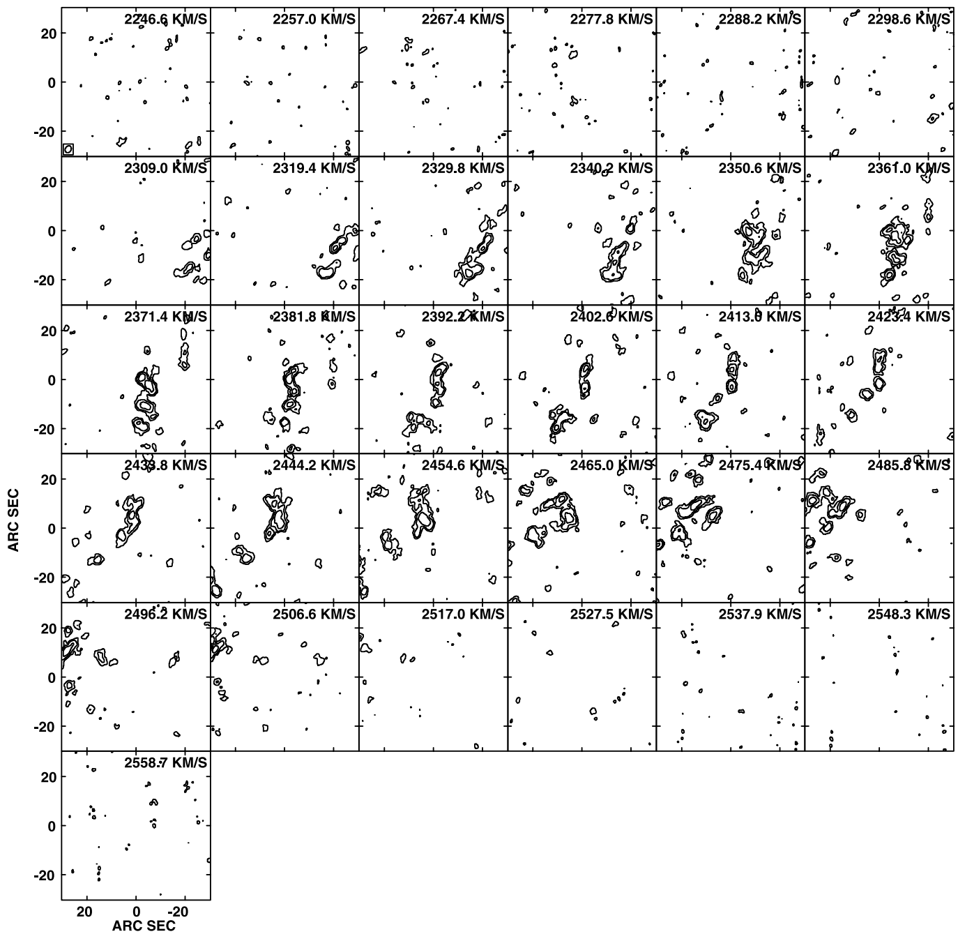
Fig. A1. (Continued.) NGC 4254: Lowest \sigma = 0.5 K.
