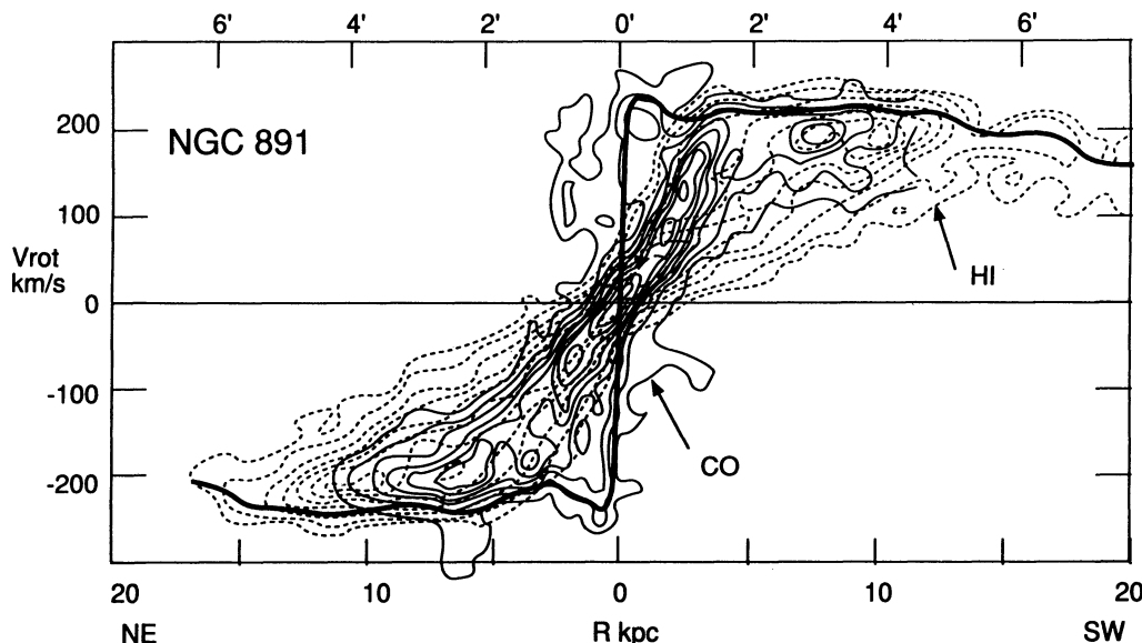
FIG. 1.—CO + H I composite position-velocity diagram for NGC 891 as reproduced from Sofue et al. (1994). A rotation curve is superposed by the thick line.
