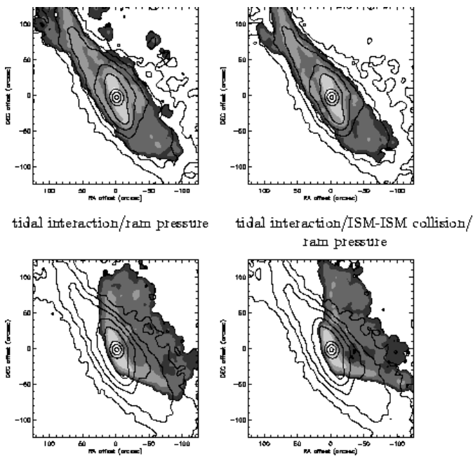
Fig. 9. Simulations of NGC 4438. Contour: stellar distribution. Greyscale: gas distribution at a resolution of 7'' . The dark regions correspond to low surface density gas.
