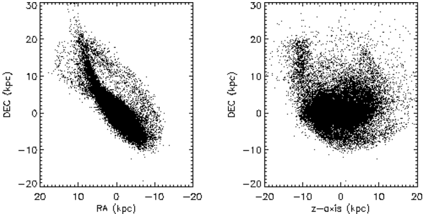
Fig. 8. Final snapshot of the stellar content at t = 260 Myr. Left panel: projected with the position and inclination angle of NGC 4438. Right panel: Perpendicular view.
