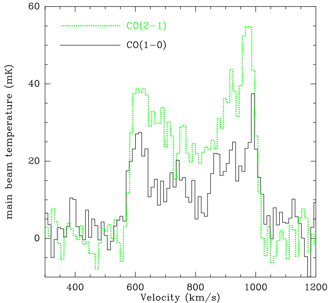
Fig. 2. CO(1–0) and CO(2–1) spectra of NGC 4435. The systemic velocity of NGC 4435 is 800 km s -1 .
