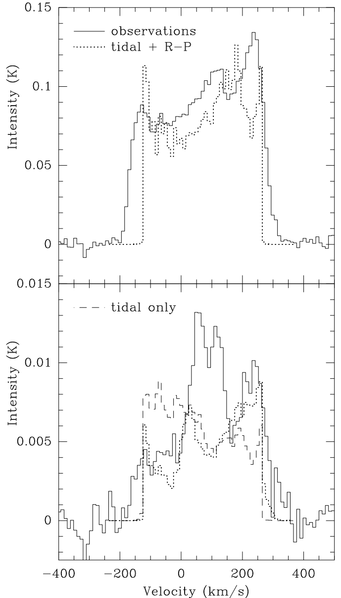
Fig. 14. Upper panel: central spectrum. Lower panel: integrated spectrum of the entire galaxy. Solid line: observed spectrum. Dotted line: model spectrum of the simulation including a tidal interaction and ram pressure stripping. Dashed line: model spectrum of the simulation including a tidal interaction alone. The systemic velocity of NGC 4438 is 70 \text{ km s}^{-1} .
