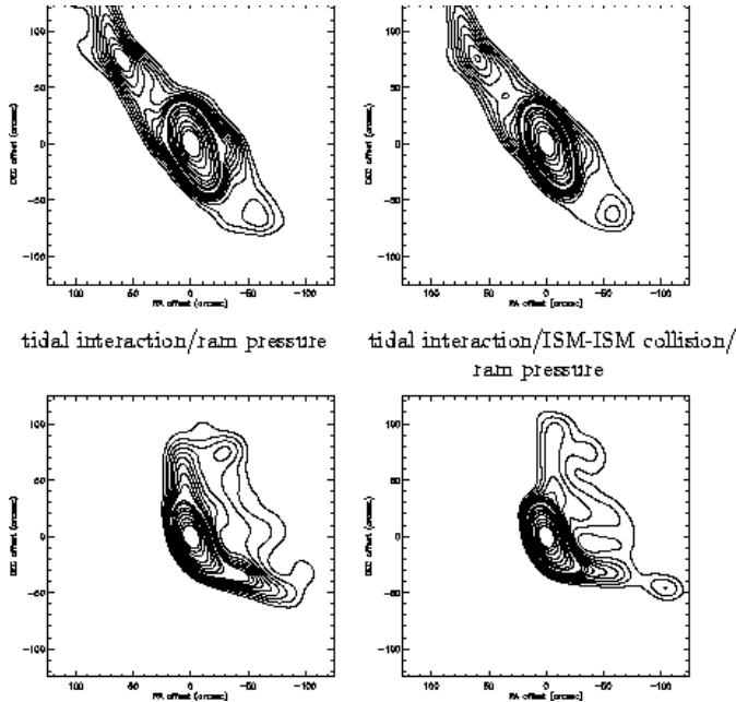
Fig. 11. Column density maps of the simulations. The contour levels are the same as for Fig. 10.
