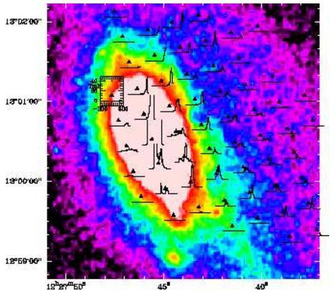
Fig. 17. Tidal interaction, ISM-ISM collision and ram pressure stripping. Simulated CO(1–0) spectra of the central part of NGC 4438 on an optical B band image. The systemic velocity of NGC 4438 is 70 \text{ km s}^{-1} .
