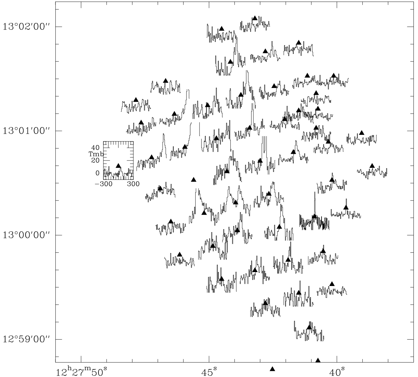
Fig. 3. Observed CO(1–0) spectra of the central part of NGC 4438 on an optical B band image. The systemic velocity of NGC 4438 is 70 \text{ km s}^{-1} .
