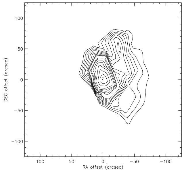
Fig. 10. Column density map of the CO(1–0) observations.
