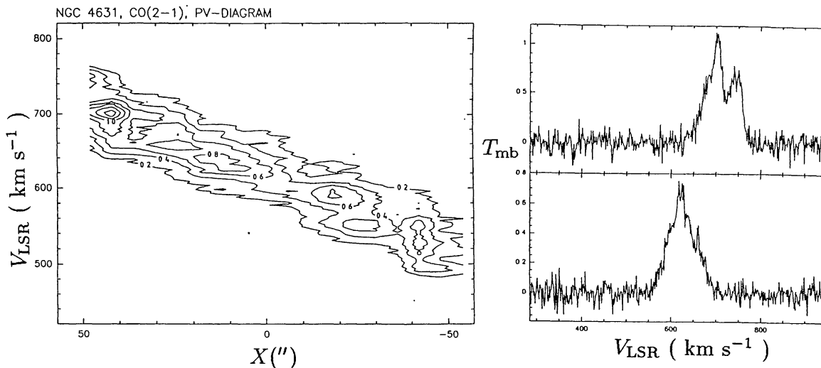
Fig.1: Position-velocity diagram of CO (2-1) line emission for NGC 4631. Note a ring at X = 1 kpc and its rigid rotation.
