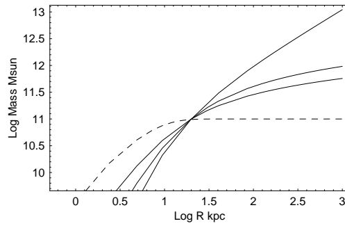
Fig. 21. Enclosed masses of dark halos up to 1 Mpc (isothermal, Burkert and NFW from top to bottom at 1 Mpc), compared with the disk mass (dashed line) that approximately manifests the galactic luminous mass.
