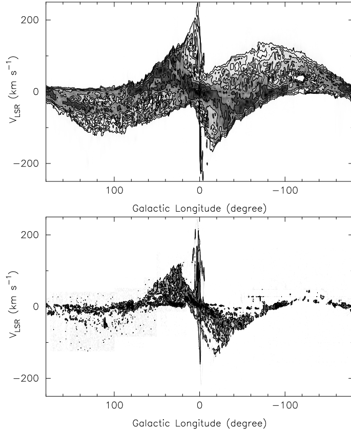
Fig. 2. Longitude-radial velocity ( l - V_{\text{lsr}} ) diagram of the \lambda 21\text{-cm} HI line emission (top: Nakanishi 2007) and \lambda 2.6\text{-mm} CO (bottom: Dame et al. 1987) lines along the galactic plane.
