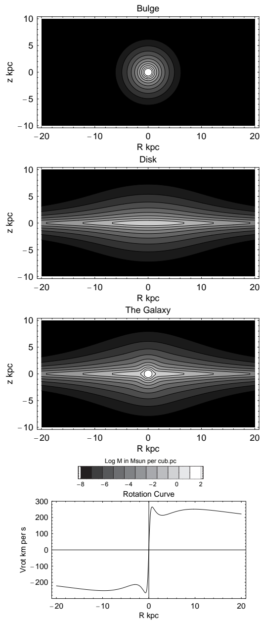
Fig. 14. Meridional distributions of the volume density in the bulge, disk and their superposition to represent the Galaxy calculated for the Miyamoto-Nagai potential (1975) with parameters in table 4. Contours and grey scales are logarithmic. The corresponding rotation curve is shown at bottom.
