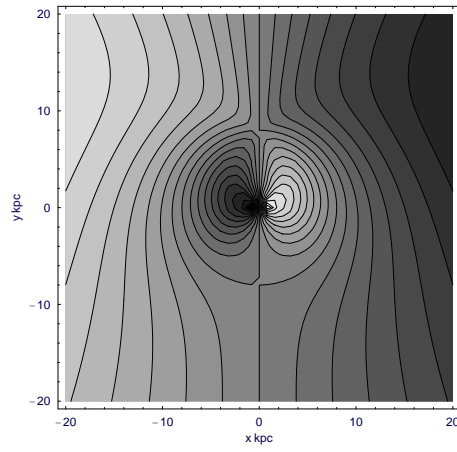
Fig. 18. Radial-velocity field in the galactic plane.
