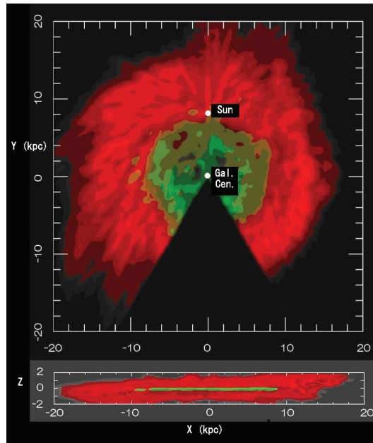
Fig. 18. Radial-velocity field in the galactic plane.
