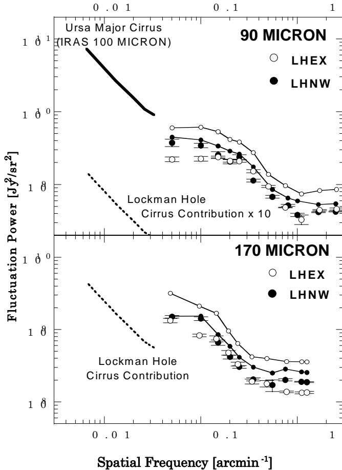
Fig. 2. Fluctuation power spectral densities (PSDs) of 90 \mu\text{m} (top) and 170 \mu\text{m} (bottom) images. Open circles represent PSDs of LHEX and filled circles represent PSDs of LHNW. As well as the PSDs of the original images (Fig. 1) shown by circles connected by thin-solid lines, the PSDs of the residual images (‘‘residual PSDs’’, where the pixels containing bright sources above 150 mJy (90 \mu\text{m} ), 250 mJy (170 \mu\text{m} ) are masked, are also shown by circles alone. The brightest source (IRAS F10597+5723) located in LHEX significantly contributes to the PSDs of the LHEX images. The 1\sigma error bars, shown only for the residual PSDs, represent the standard deviation in a set of the PSDs with different position angles in the sky. Thick line is an example of the IR cirrus PSD, which is an average spectrum of several IR cirrus in Ursa Major, with 100 \mu\text{m} brightness of 2–3 MJy/sr. Dotted lines are the IR cirrus PSDs in the Lockman Hole, estimated by assuming that the cirrus PSDs are proportional to B_0^3 , where B_0 is mean brightness of the cirrus cloud.
