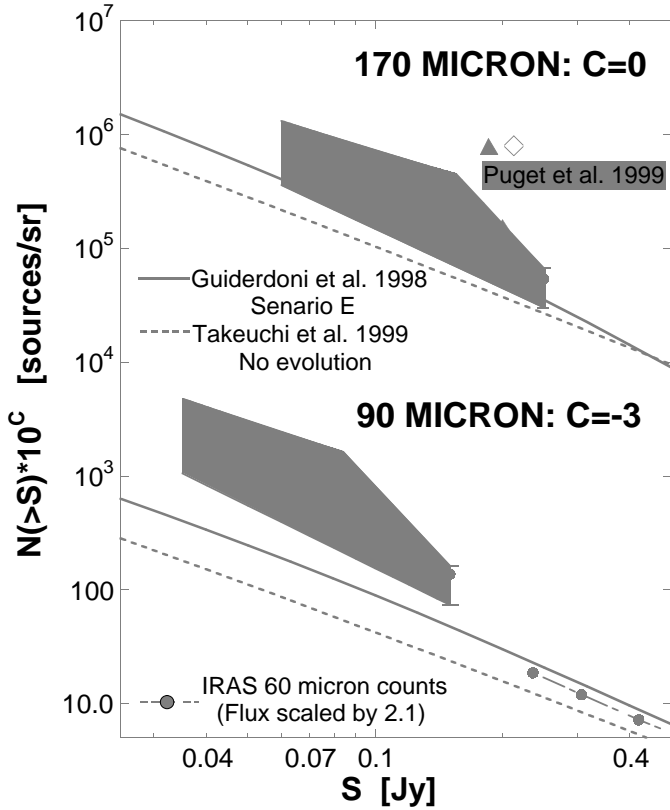
Fig. 4. The shaded areas show the allowed regions for various number count models, which are consistent with the fluctuation powers of the Lockman Hole images (Fig. 3). The bottom border is obtained from the simple number count model with a single power-law index between S_{\min} = 1 mJy and S_{\max} = 150 mJy ( 90 \mu\text{m} ) or 250 mJy ( 170 \mu\text{m} ). The upper border is determined from the allowed double power-law count models. See text for detailed information. The filled circles are observed number counts at S_{\max} . The theoretical number count models by Guiderdoni et al. (1998) (scenario E: solid lines) and the no evolution model by Takeuchi et al. (1999) (dashed lines) are also shown. The open diamonds and triangles are observed and incompleteness-corrected source counts obtained by the FIRBACK Marano 1 survey (Puget et al. 1999). The open circles with dash-dotted line show the IRAS 60 \mu\text{m} counts, in which the flux is scaled by the factor S_{\nu}(90 \mu\text{m})/S_{\nu}(60 \mu\text{m}) = 2.1 .
