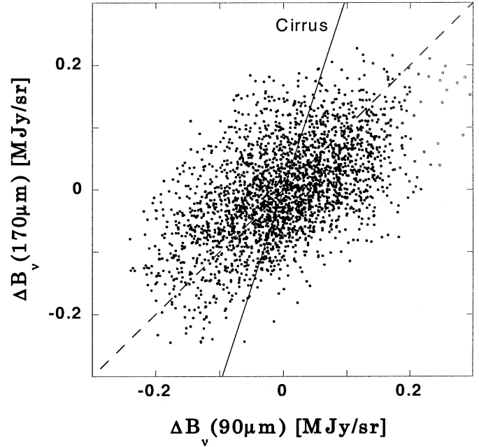
Fig. 5. Point-to-point comparison between the 90 \mu\text{m} sky brightness and the 170 \mu\text{m} one in the Lockman Hole. The brightness is not absolute one, but is offset from the median brightness. In this plot the pixels around the bright sources ( S \geq 150 mJy for 90 \mu\text{m} , S \geq 250 mJy for 170 \mu\text{m} ) are not shown. In order to avoid the error due to the difference of the beam size between the two bands, the 90 \mu\text{m} images are convoluted with the 170 \mu\text{m} beam profile ( 144'' FWHM). The solid line showing the IR cirrus color vector is taken from Lagache et al. (1999), which is 17.5 K gray-body with an emissivity proportional to \lambda^{-2} .
