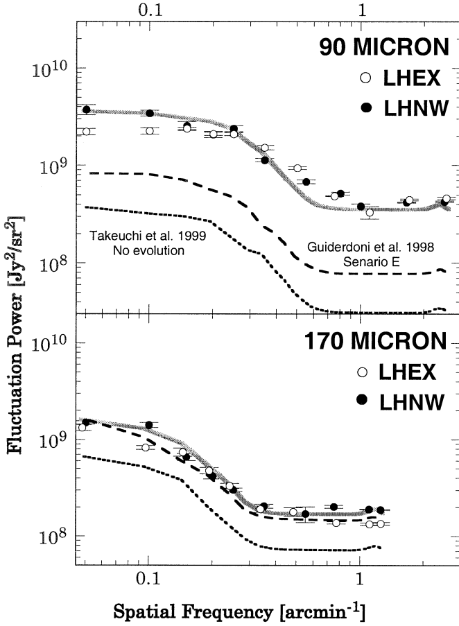
Fig. 3. The residual PSDs of 90 \mu\text{m} (top) and 170 \mu\text{m} (bottom) images (open circles and filled circles, same as Fig. 2) are compared with the simulated PSDs based on various number counts models: dashed lines are PSDs of the simulated images by Guiderdoni et al. (1998) scenario E, while the dotted lines are those by Takeuchi et al. (1999) no-evolution. Thick gray lines are examples of the simulated images produced by simple double power-law number count models (see text for details).
