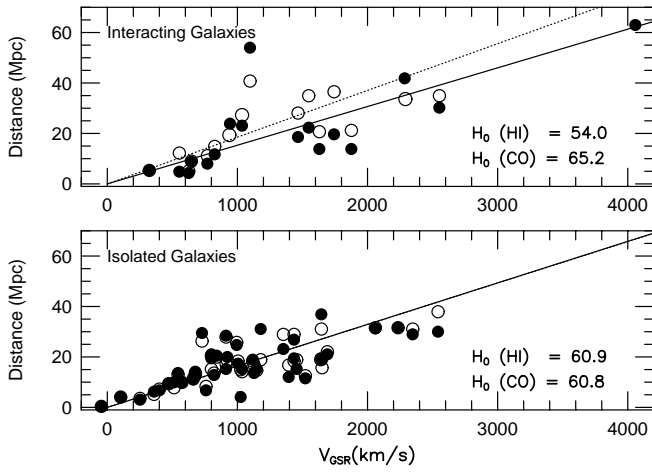
Fig. 3. Hubble diagrams for interacting galaxies (top) and isolated galaxies (bottom), radial velocities referred to the Galactic Standard of Rest (from RC3) versus distances derived from the Tully-Fisher relation. Symbols are the same as in Fig. 1. Distances derived from the CO linewidths are plotted by filled symbols and those derived from the HI linewidths are plotted by open symbols. The solid and dotted lines indicate the regression lines of the CO and HI data, respectively.
