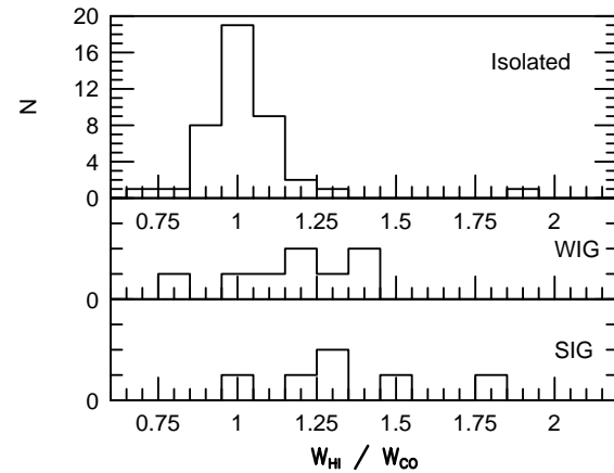
Fig. 2. Histograms of W_{\text{HI}}/W_{\text{CO}} for isolated galaxies (top), weakly interacting galaxies (middle) and strongly interacting galaxies (bottom).
