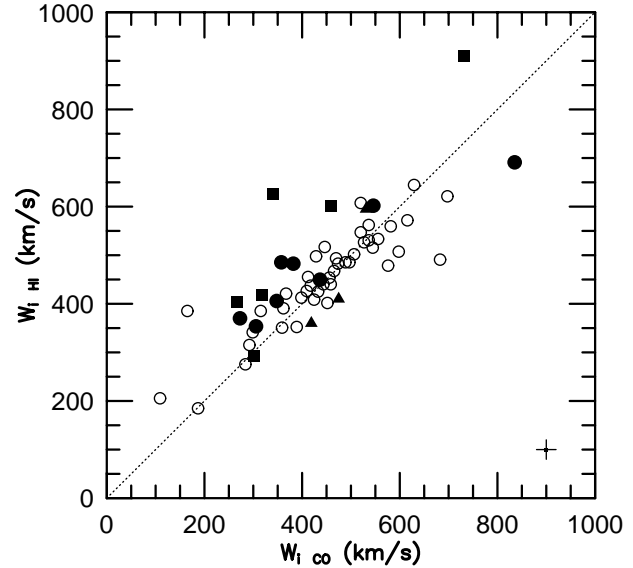
Fig. 1. The CO linewidths versus the HI linewidths corrected for inclination. Isolated galaxies are marked by open circles. Interacting galaxies are marked by filled symbols; mergers by filled triangles, SIG by filled squares, and WIG by filled circles. The subclasses of the interacting galaxies are explained in Sect. 2.
