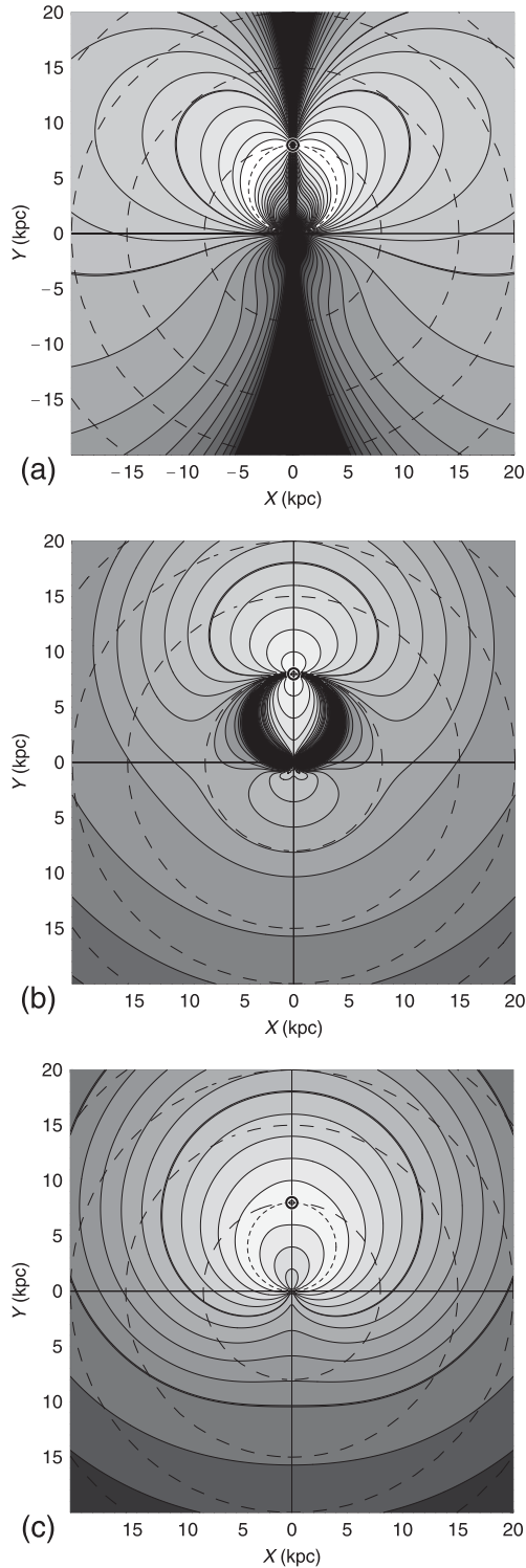
Fig. 5. (a) Accuracy diagrams \Delta V_{\text{rot}}^v(X, Y) for \delta v_r = 1 \text{ km s}^{-1} and \delta r/r = 0.02 (2% distance error), (b) \Delta V_{\text{rot}}^\mu(X, Y) for \delta \mu = 0.2 \text{ mas yr}^{-1} , and (c) \Delta V_{\text{rot}}^{\text{ec}}(X, Y) for \delta v_p/r = 1 \text{ km s}^{-1} \text{ kpc}^{-1} corresponding to \delta \mu = 0.21 \text{ mas yr}^{-1} , \delta v_r = 1 \text{ km s}^{-1} , and \delta r/r = 0.02 (Sofue 2011).
