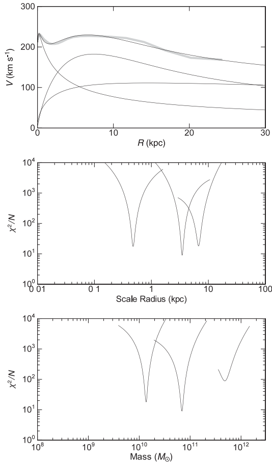
Fig. 30. Rotation curve and \chi^2 -fitting result for NGC 891 (top), the distribution of \chi^2/N around the best-fitting scale radii (middle), and the masses (bottom) of the three components.
