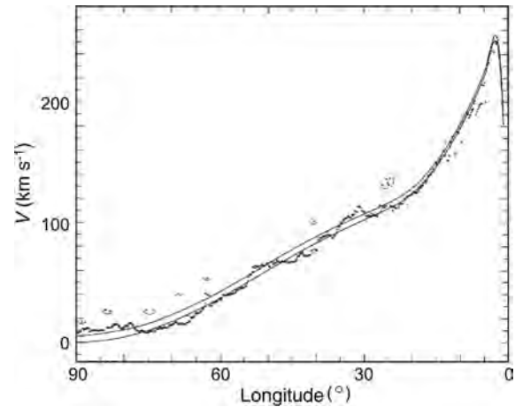
Fig. 2. CO and H I line tangent velocities for the inner rotation curve (Burton & Gordon 1978).
