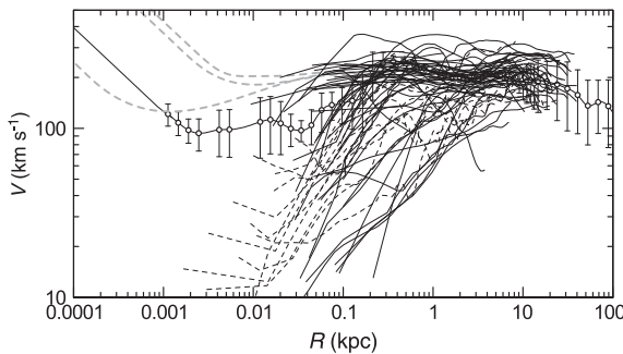
Fig. 19. Logarithmic rotation curves of nearby spiral galaxies with typical resolutions, \sim 2'' – 10'' (thick lines) and those from Virgo CO survey ( \sim 1'' , thick dashed lines), compared with the Milky Way rotation curve (circles with error bars). Three thick-dashed lines show NGC 224, NGC 1068, and NGC 4258 as interpolated with their black holes by horizontal straight lines.
