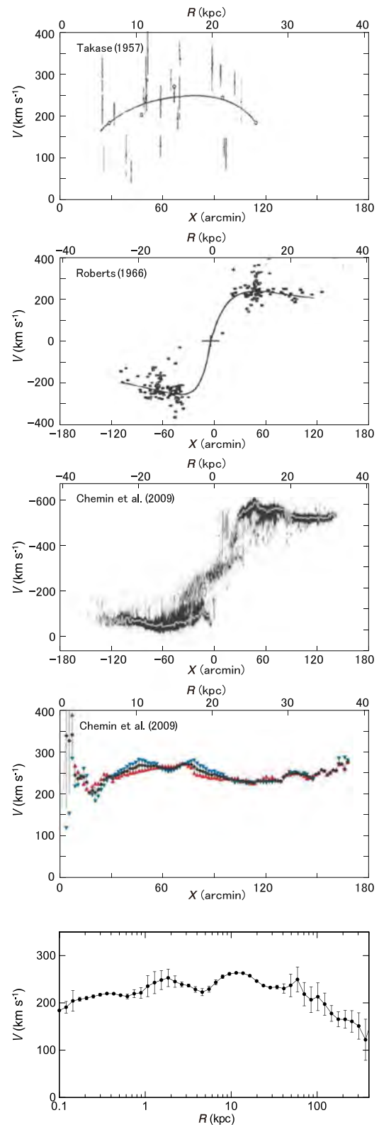
Fig. 8. Half a century of progress in the rotation curve of M31. From top to bottom: 1950s— a rotation curve using data obtained by M.U. Mayall et al. in the 1940s (Takase 1957); 1960s—rotation curve in the H I 21 cm line (Roberts 1966); a modern position–velocity diagram and a rotation curve in H I, showing flat rotation up to 40 kpc (Chemin et al. 2009); and a grand rotation curve from the center to ~300 kpc in semi-logarithmic scaling (Sofue 2013b). (Color online)
