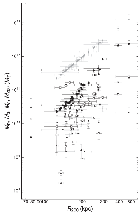
Fig. 32. Size–mass relations for (R_{200}, M_b) (triangles); (R_{200}, M_d) (rectangles); (R_{200}, M_h) (black dots); and (R_{200}, M_{200}) (small gray dots), showing the trivial relation by definition of the critical mass.
