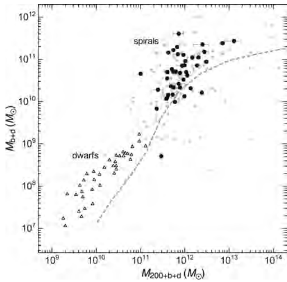
Fig. 33. M_{b+d} – M_{200+b+d} relation compared with the stellar mass–total mass relation for dwarf galaxies (triangles: Miller et al. 2014) and simulation + photometry (dashed gray line: Behroozi et al. 2013). Black dots are the selected galaxies with reasonable fitting results, while small gray dots as well as black dots show non-weighted results from automatic decomposition of all rotation curves.
