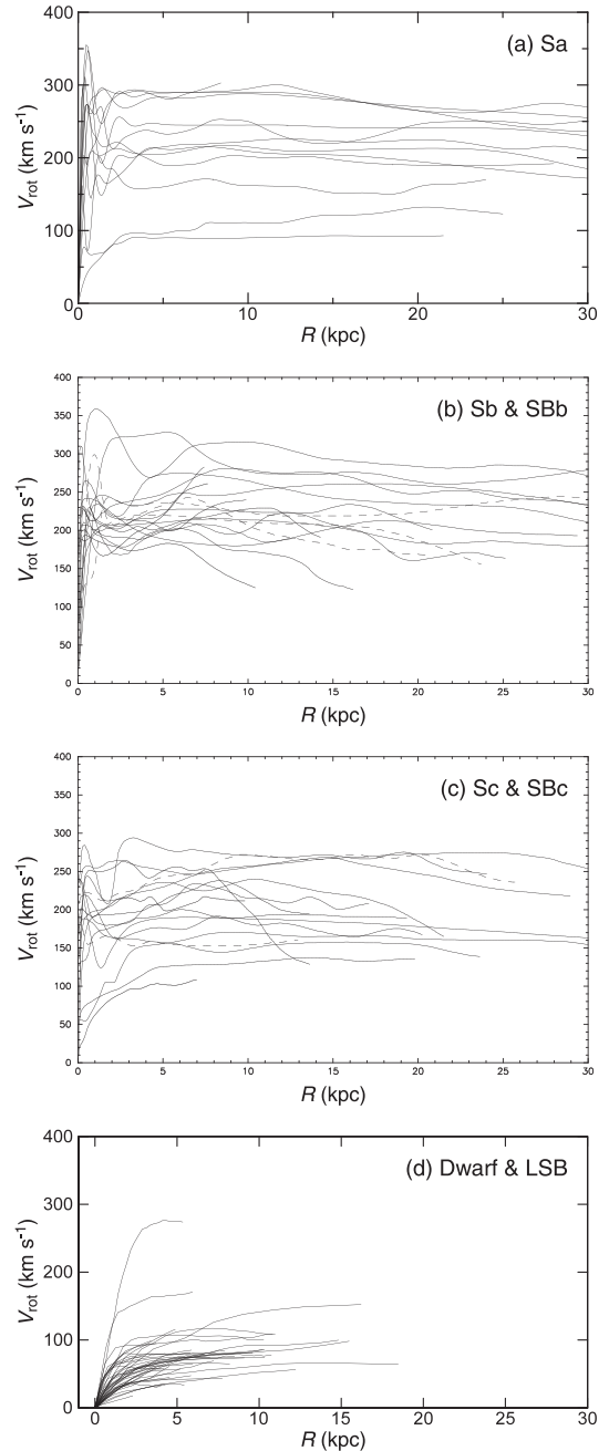
Fig. 15. Rotation curves for Sa-type galaxies (top: Noordermeer et al. 2007), Sb (solid lines) and barred SBb (dashed lines) (second panel), Sc (solid line) and SBc (dashed lines) (third panel: Sofue et al. 1999), and dwarf and low surface brightness galaxies (bottom: Swaters et al. 2009).
