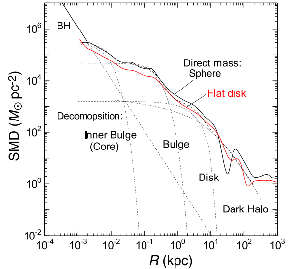
Fig. 22. Directly calculated SMD of the Milky Way under the sphere (thick black line) and flat-disk (thin red line) assumptions on a log-log plot, compared with the result found by the deconvolution method (dashed lines). The straight line represents the black hole with mass 3.6 \times 10^6 M_{\odot} . (Color online)
