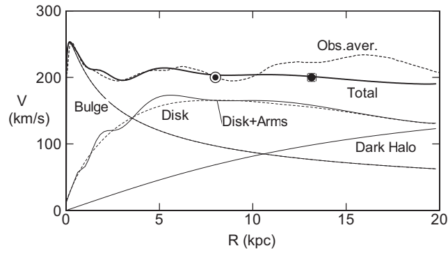
Fig. 5. Observed circular velocities representing the rotation curve of the Galaxy (Sofue et al. 2009).. Plot was obtained using HI tangent velocity data (Burton and Gordon 1978; Fich et al. 1989); CO tangent-velocity data (Clemens 1985); CO cloud + HII region + OB stars (Fich et al. 1989, Blitz et al. 1982); Late type stars (Demers and Battinelli 2007); HI thickness method (Honma and Sofue 1997). Big circle at 13.1 kpc is from VERA by parallax, radial and proper motions (Honma et al. 2007). All data have been converted to (R_0, V_0) = (8.0, 200.0 \text{ km s}^{-1}) .
